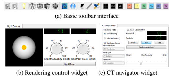
Figure 3: (a) shows the basic toolbar interface for convenient access to functions. (b) widgets for controlling the intensity of key/fill virtual lights. (c) CT medical imaging data navigation options of stack and volume rendering.
